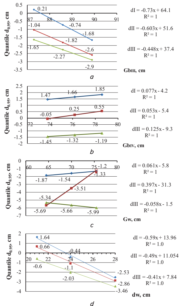
Fig. 8. Dependence of quantiles dI, dII, dIII on value of body measurements: a – Gb_{III} ; b – Gb_{IV} ; c – Gw ; d – dw
