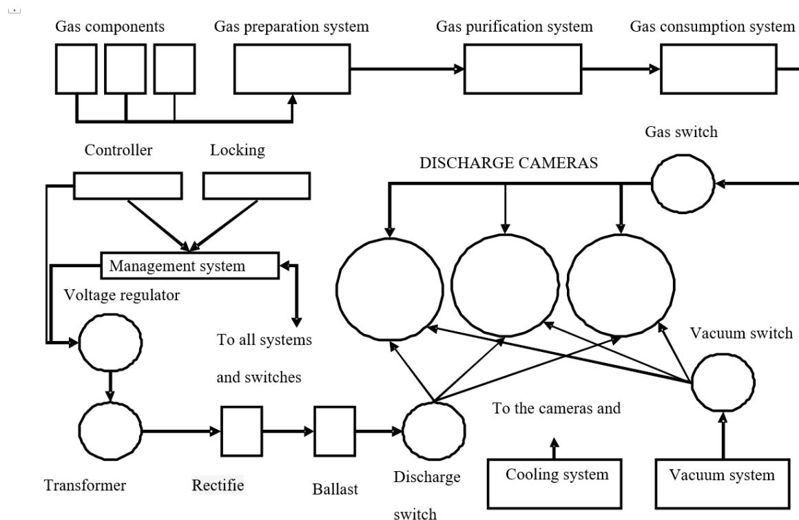
Fig. 1. Block diagram of a three-chamber installation
