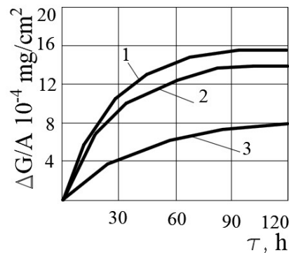
Fig. 3. Weight loss in cavitation of CEP Ni-SiC28-B in hard water:
