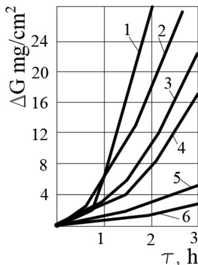
Fig. 1. Wear kinetics at micro-shock load: 1, 2 – steel 45 normalized, respectively, in 3 % NaCl solution and hard water; 3, 4 – CEP Ni-SiCano in 3 % NaCl solution and hard water; 5, 6 – CEP Ni-SiC found after annealing in vacuum in 3 % NaCl solution and hard water
