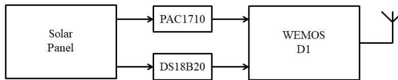
Figure 1. Solar panel intelligent monitoring system block diagram
