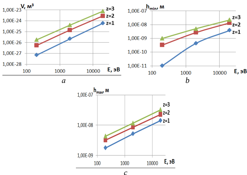
Fig. 2. Dependence of NC (a), of minimal (b) and maximal (c) depth of NC occurrence at act of ions of hafnium ( \text{Hf}^+ ) with different charge ( z = 1, z = 2, z = 3 ) for T12A
