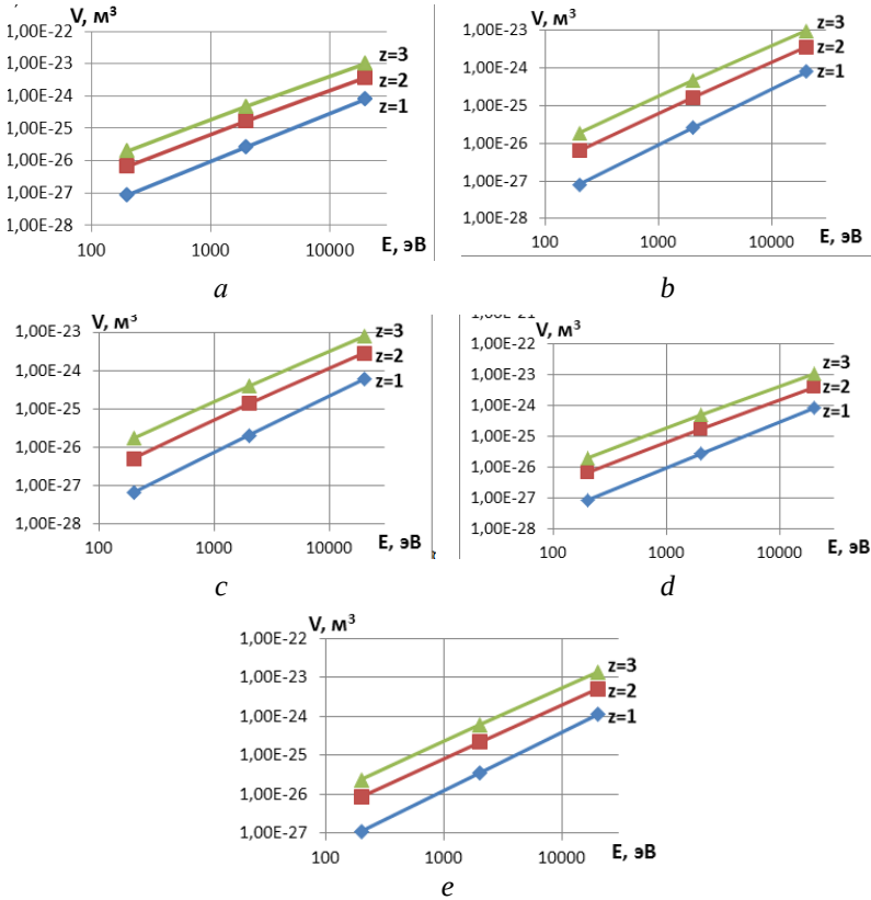
Fig. 3. Dependence of NC volume under ion effect of zirconium ( \text{Zr}^+ ) (a), molybdenum ( \text{Mo}^+ ) (b), tungsten ( \text{W}^+ ) (c), yttrium ( \text{Y}^+ ) (d) and nickel ( \text{Ni}^+ ) (e) with different charges ( z = 1, z = 2, z = 3 ) for T12A
