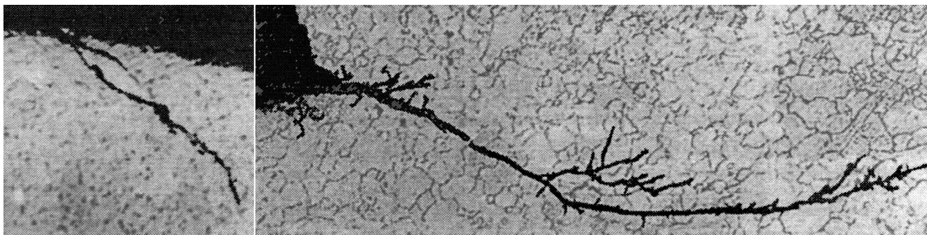
Fig. 2. Origination and propagation of micro-cracks in the surface coating of the gear, x500
