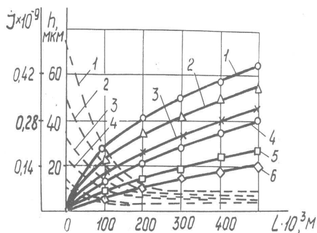
Fig. 5. Kinetics of steel wear 45H in oil I-20 at a specific pressure of 4MPa and a sliding speed of 1 m/s: 1-was to improve; 2, 3, 4-nitriding steel (100% \text{N}_2 , P=265 Pa, \tau=4 hours) at temperatures of 520, 560 and 600°C respectively; 5, 6-nitrided steel ( T=560^\circ\text{C} 75 vol.% \text{N}_2 +25 vol.% Ar, \tau=4 hours) at a pressure of gaseous medium 450 and 80Pa respectively
