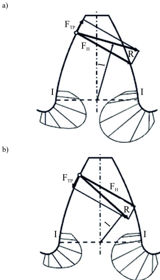
Fig. 1. Shoulder application of the resultant force R on the action of the normal force and frictional force F_H for driving the F_{TP} (a) and slave (b) of the teeth in the dangerous section
