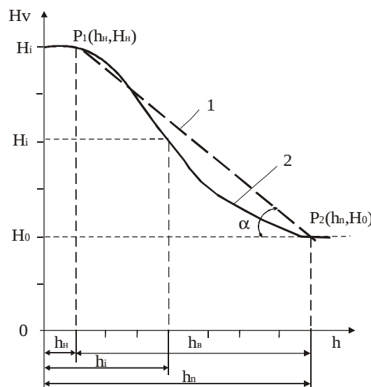
Fig. 1 – Distribution of hardness through the thickness of the nitrided layer: 1 – on linear dependence; 2 – by an exponential dependence
