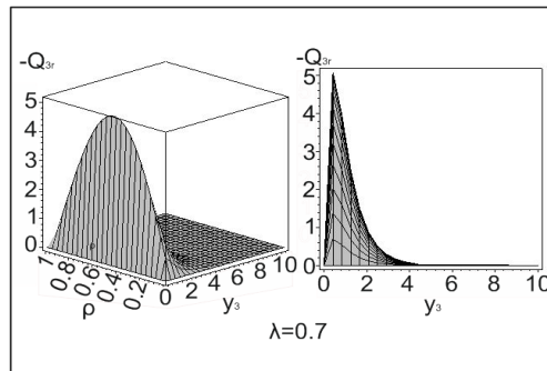
Fig. 6. Tangential stresses (Treloar potential)
