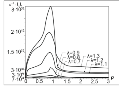
Fig. 5. Move U_r in the elastic layer (harmonic potential)
