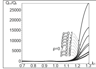
Fig. 3. Effect of initial stresses on normal distribution law (harmonic potential)
