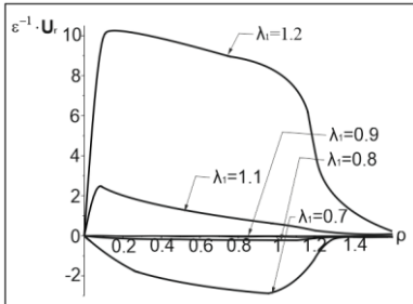
Fig. 4. Displacement U_r in the elastic layer (Treloar potential)
