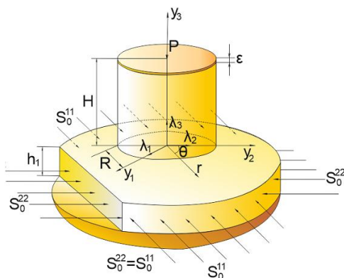
Fig. 1. Cylindrical stamp, layer and base with initial stresses
