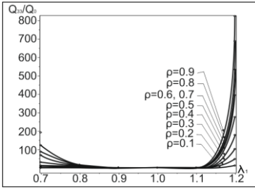
Fig. 2. Effect of initial stresses on the normal law of distribution (Treloar potential)
