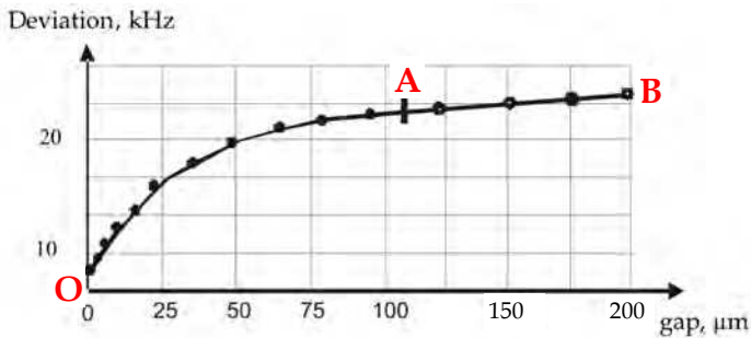
Fig. 4. Graduation characteristic of PRMT with MIG
