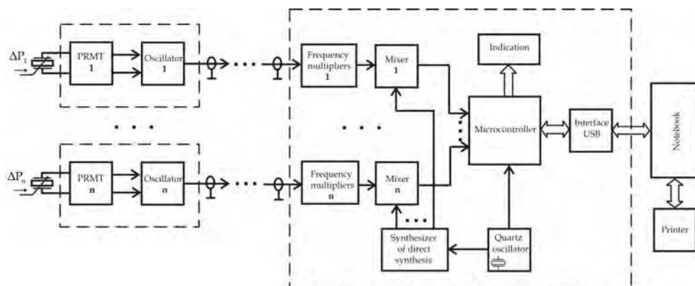
Fig. 23. Structure of sphygmographic system BIOTON
