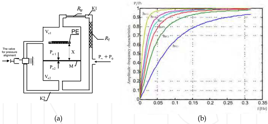
Fig. 16. (a) Pneumatic scheme of PRMT; (b) The amplitude- frequency characteristics of sensor of pressure for values l_{tr} = 1 \text{ mm}
