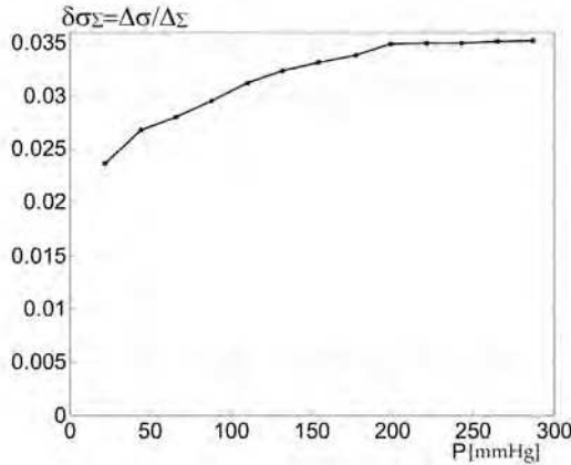
Fig. 21. The relative characteristic of sensitivity
