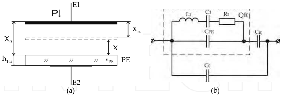
Fig. 3. (a) PRMT with MIG design map; (b) Equivalent electric circuit of PRMT
