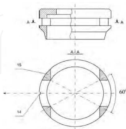
Fig. 20. The construct of quartz holder
