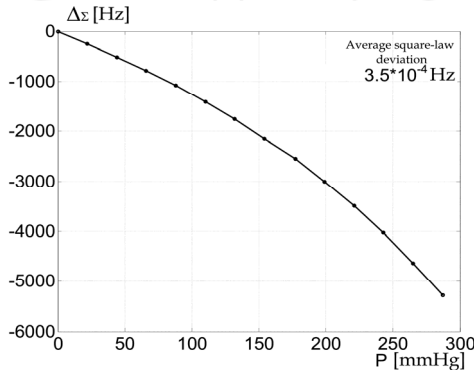
Fig. 18. Summarized modulation characteristic for PMRT with PM
