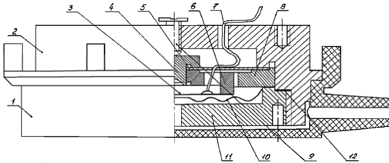
Fig. 15. Construction of PMRT with metal membrane
