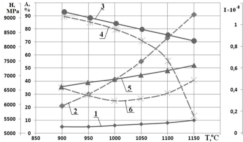
Fig. 4. Characteristics of steel 5 after nitriding (continuous line) and nitrohardening (dashed line): 1 - 2 – austenite content; 3 - 4 – microhardness of the surface layer; 5 - 6 – wear intensity after friction way 3 \times 10^3 m
