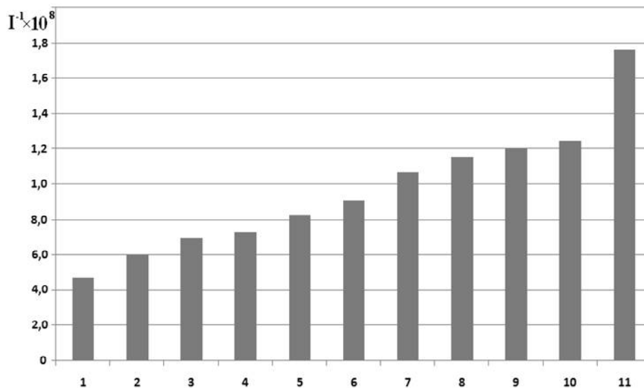
Fig. 5. Diagram of different steels wear at abrasive wear in model solutions with different thermal and chemical-thermal treatment:
