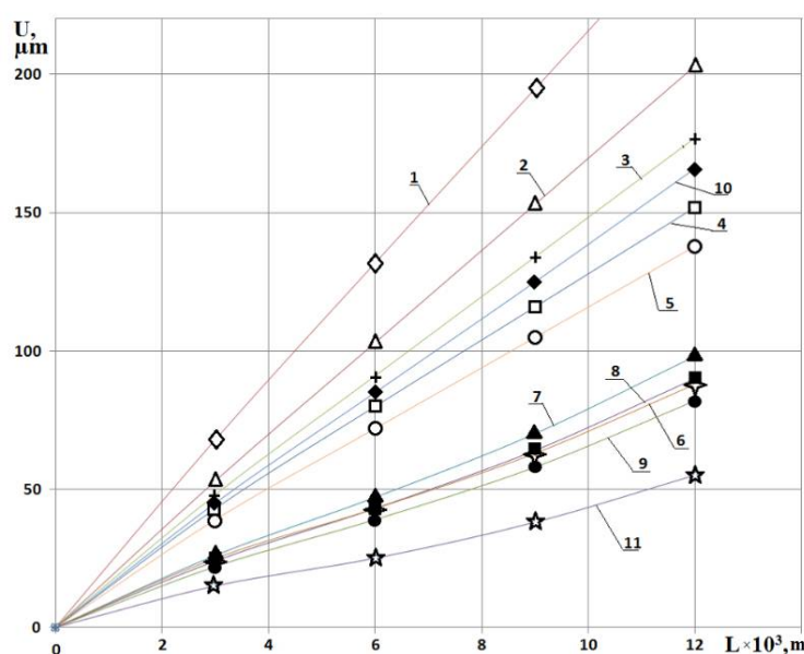
Fig. 1. The dependence of wear of different steel samples on friction way:
