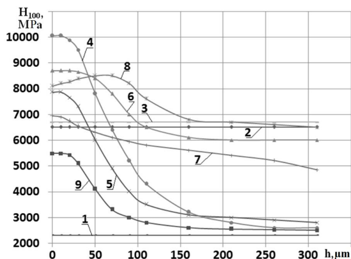
Fig. 3. Hardness distribution in the depth of surface layer at different thermal and chemical-thermal treatment:
