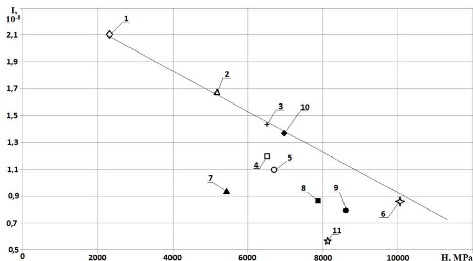
Fig. 2. Wear intensity of different steels in model medium after 12 \times 10^3 m friction way:
