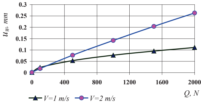
Fig. 8. Effect of sliding velocity and load on wear of the slide bearing
