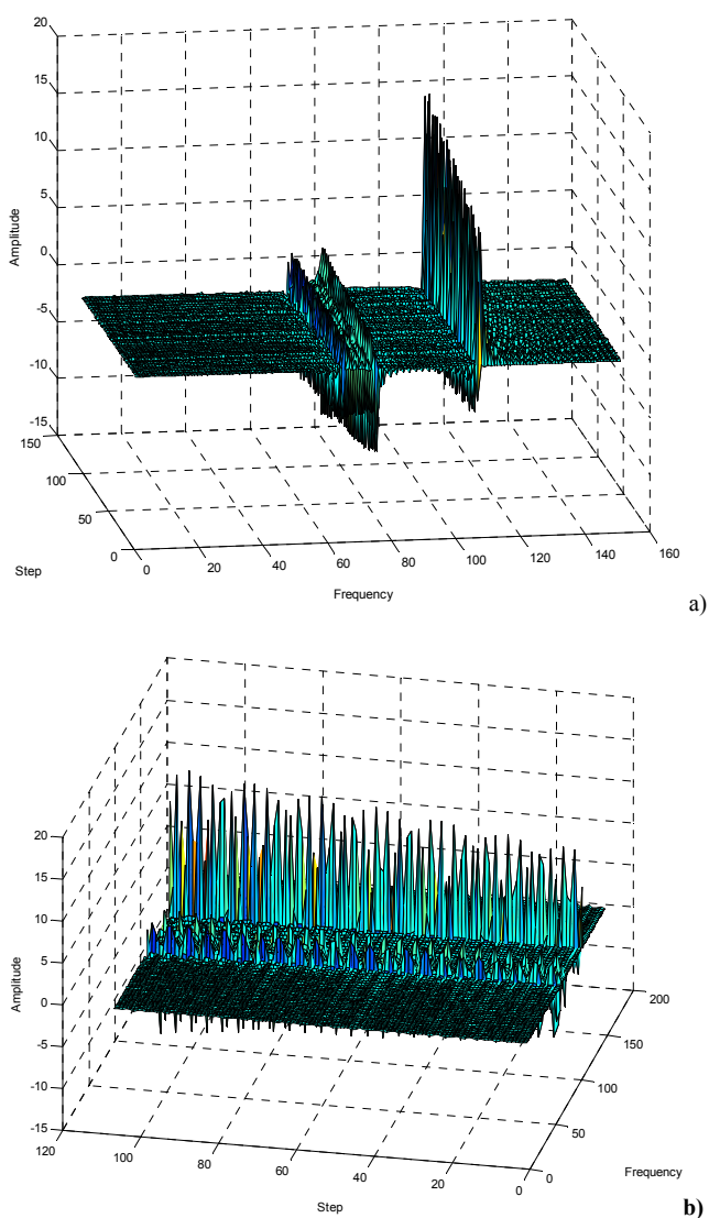
Fig. 3. A result of spectrology of signal is after setting of norms with application of the offered algorithm
