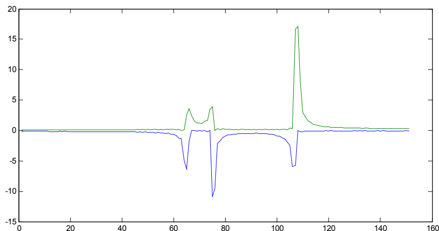
Fig. 4. A result of total accumulation of spectral constituents of got is at DFT with the different after a windows width
