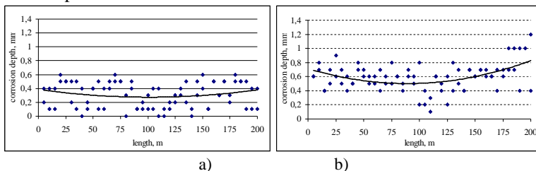
Fig. 2. Data of corrosion depth on the bottom of the ship hull line „A“: a) after 20 years of exploitation; b) after 25 years of exploitation.
