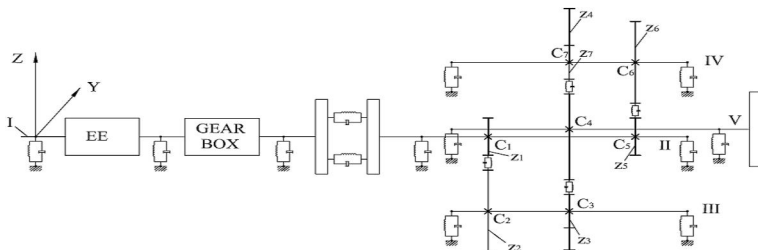
Fig. 3 The dynamic model of rotating system [1, 2]
