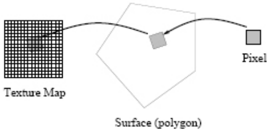
Fig.1. Texture mapping: map pixel onto polygon and then into texture map[3]
