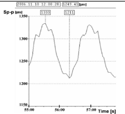
Fig. 2. The rotor II with z_4 radial displacement plot, s_{p-pR} = 133 \mu\text{m} value, full rotation at 87 s
