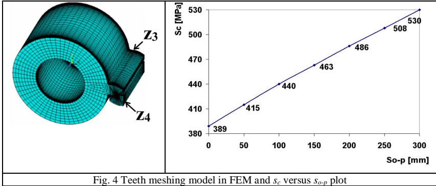
Fig. 4 Teeth meshing model in FEM and s_c versus s_{o-p} plot
