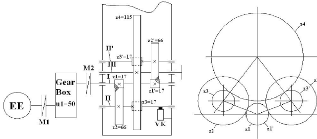
Fig.1. Heavy duty gear power transmission
