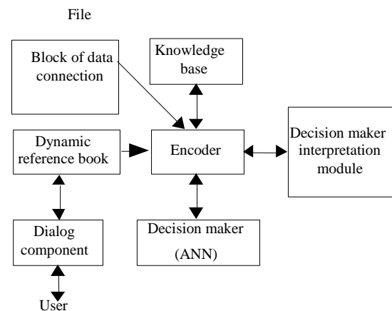
Fig.1. Structure chart of repeated software testing system
