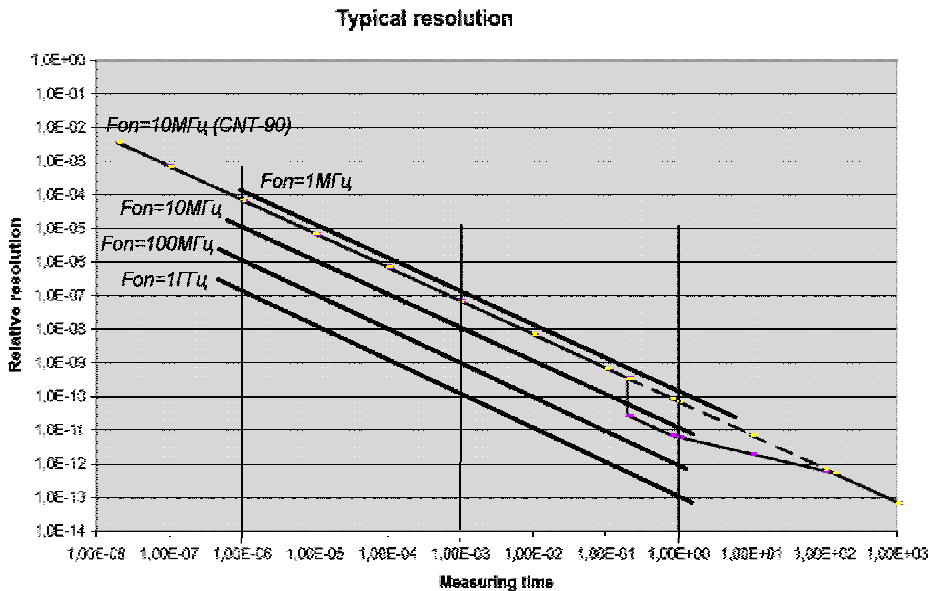
Figure 8: Comparison of coincidence frequency-meter with "the best in the world" frequency-meter CNT-90
