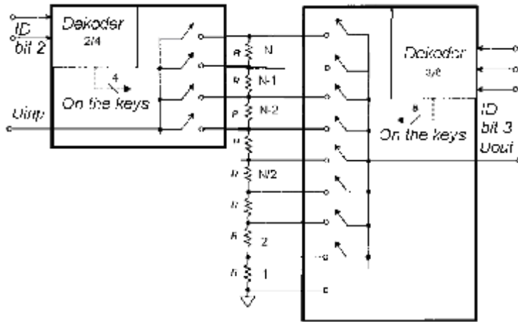
Figure 2: Divider-attenuator circuit of Trotsyshyn for 8R
