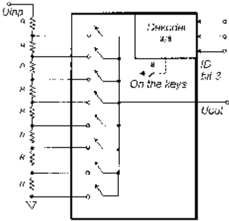
Figure 1: . Divider Kelvin
