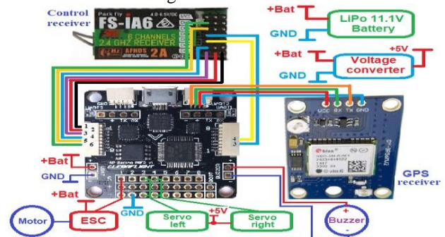
Fig. 2. The wiring diagram for the electronic components of the wing
