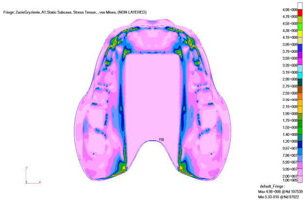
Fig. 3. Stress map for polyamide and 6% glass fibre
