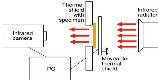
Fig. 1. Scheme of the experimental arrangement
