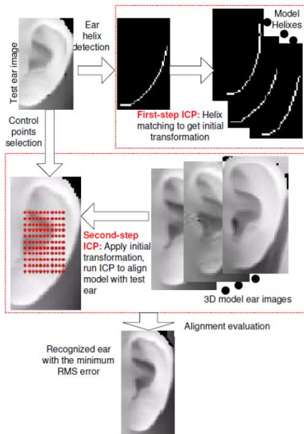
Fig.1. System diagram with ICP algorithm
