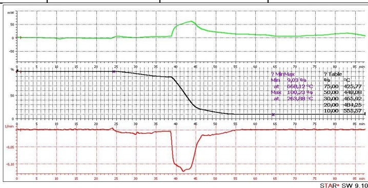
Fig.2. Example curve for polyethylene with 10% content of bentonite
