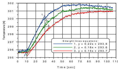
Fig. 3. Maximal temperature variations versus time for carbon/epoxy specimens including: 1. 23wt.%, 30wt.%, 3. 37wt.% carbon content
