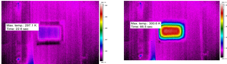
Fig. 2. Thermal images of 23wt.% carbon fiber specimen captured on the opposite side to the heated surface after: 22.6 and 66.5 seconds counting from the beginning of the heating process
