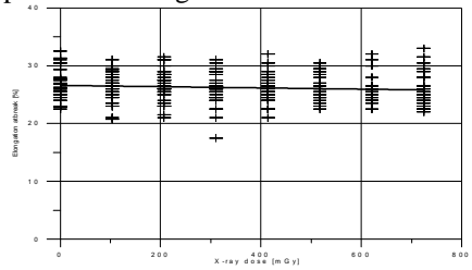
Fig.4. Dependence of elongation at break on impulse X-ray dose for polyester yarn before sterilization
