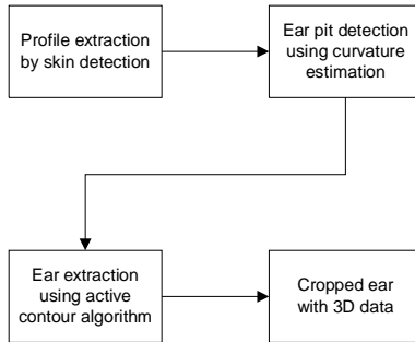
Fig. 2. Scheme of automatic ear extraction
