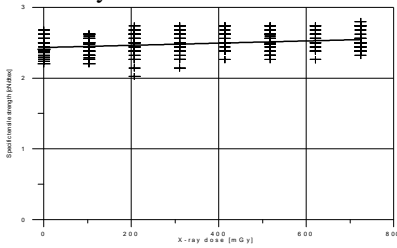
Fig.3. Dependence of specific tensile strength on X-ray dose for polyester yarn before sterilization
